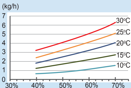
Dehumidification Capacity Chart
